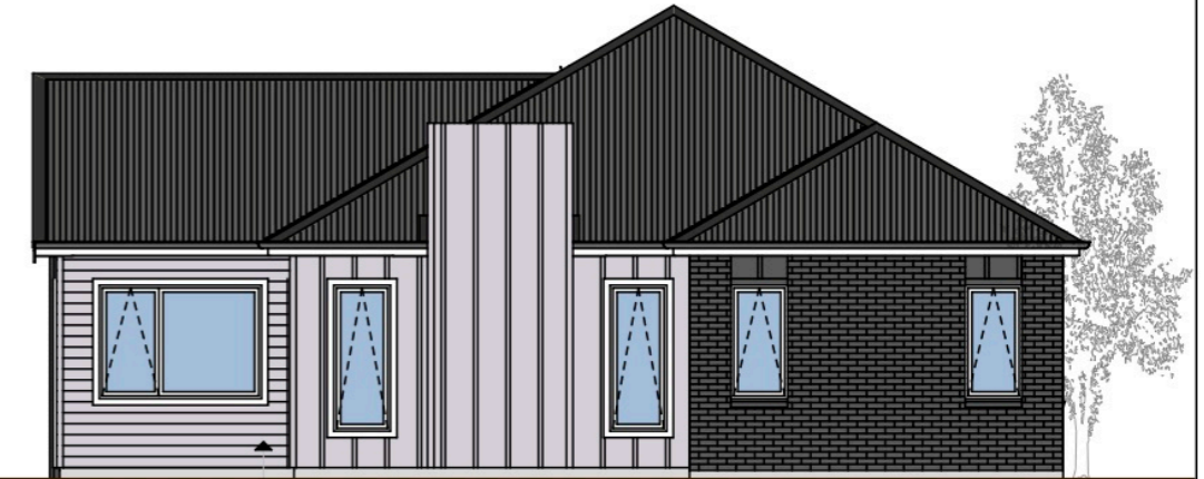
ELEVATION 2 (WESTERN)
